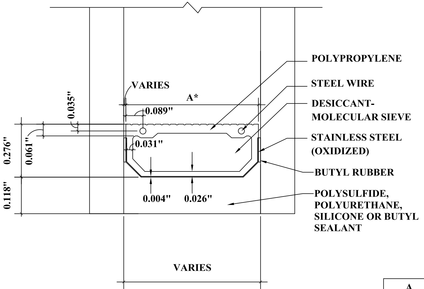
DETAIL FOR THERMAL MODELING OF ENSINGER THERMIX TX.N PLUS SPACER (TS-D)
